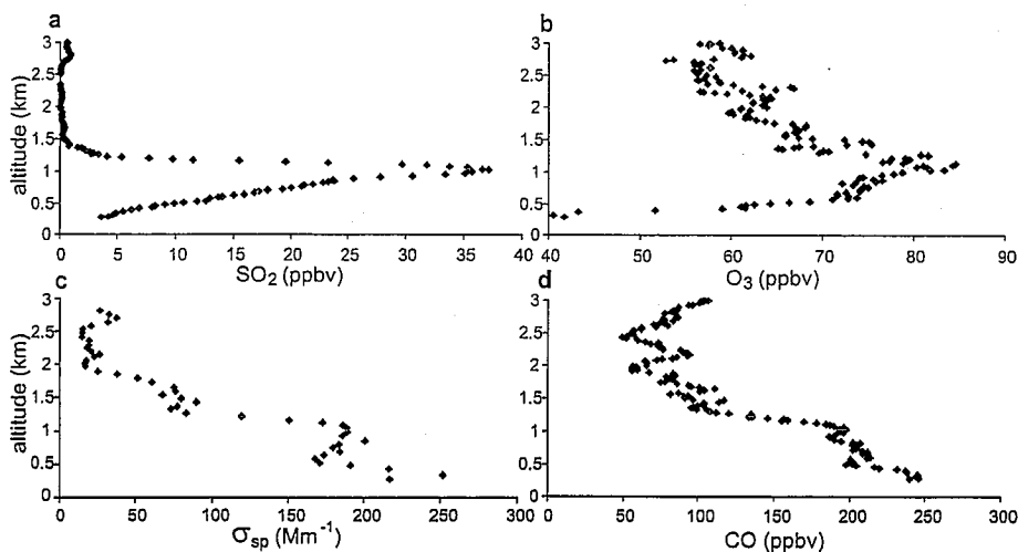
Figure 1. Running 1 min mean \text{SO}_2 mixing ratios (a); 10 s \text{O}_3 mixing ratios (b); particle light scattering at 550 nm (c); and running 1 min mean CO mixing ratios (d) over Luray, Virginia (outside blackout area) at 1400 UTC (10:00 LST) 15 Aug, 2003.
