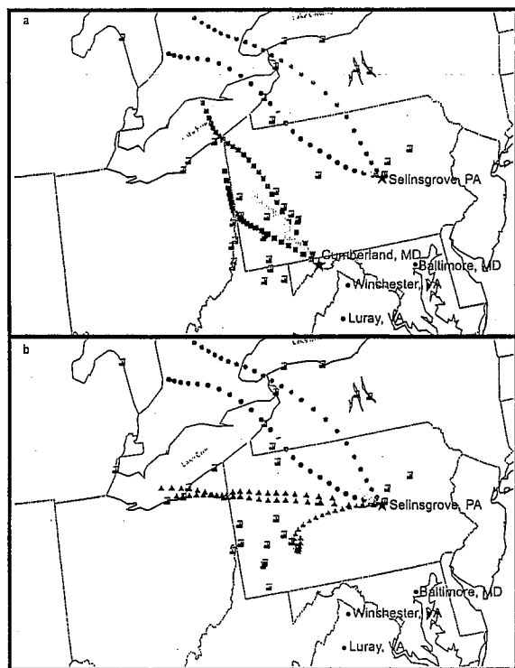
Figure 3. Map of northeastern U.S. showing modeled back trajectories (24 h) from Cumberland, MD and Selingsrove, PA on 15 Aug, 2003 at 1500 and 2000 UTC, respectively (a); and Selingsrove, PA on 15 Aug, 2003 (circles) and on 4 Aug, 2002 (triangles) at 2000 and 2100 UTC, respectively (b). Light gray represents 0–500 m, dark gray 500–1500 m, and black 1500–2500 m AGL. Icons represent power plants that fall within trajectory buffers regardless of size or extent of down scaling during the blackout.
