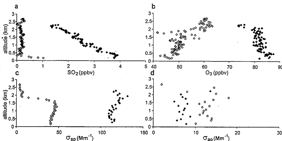
Figure 4. Comparison of running 1 min mean \text{SO}_2 mixing ratios (a); 10 s \text{O}_3 mixing ratios (b); particle light scattering at 550 nm (c); and particle light absorption at 565 nm (d) measured on 15 Aug, 2003 (open diamonds) and 4 Aug, 2002 (filled diamonds) over Selinsgrove, Pennsylvania.
