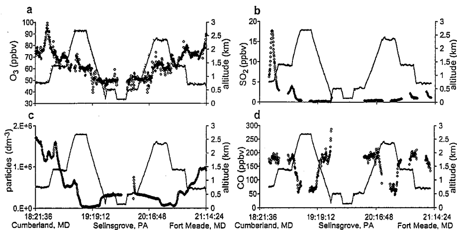
Figure 2. Second flight on August 15, 2003 showing altitude (solid black lines), time (UTC), as well as takeoff, landing and spiral locations. Open diamonds represent 10 s \text{O}_3 mixing ratios (a); running 1 min mean \text{SO}_2 mixing ratios (b); sub-micrometer particle counts (c); and running 1 min mean CO mixing ratios (d).
